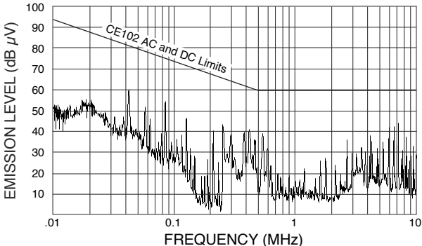
CE102: High power DC-DC converter filtered with an FMCE-0328.
