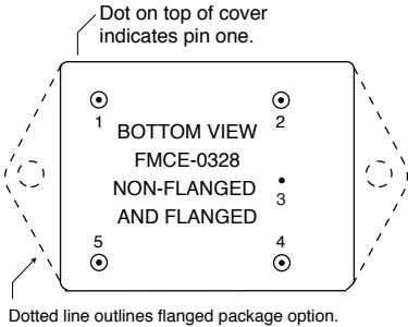
FIGURE 3: PIN OUT
