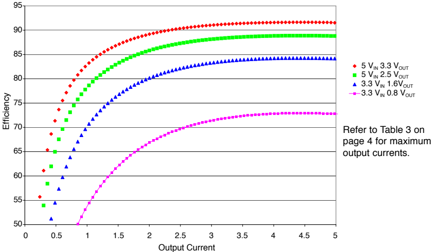
FIGURE 11: TYPICAL EFFICIENCIES
