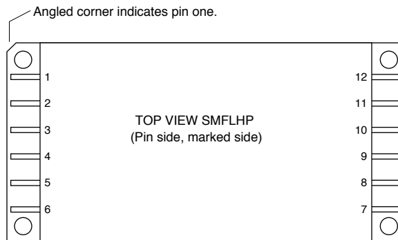
FIGURE 3: PIN OUT
