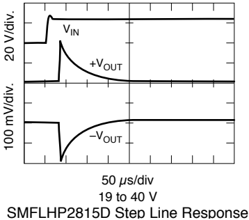
SMFLHP2815D Step Line Response
