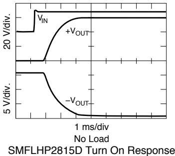
SMFLHP2815D Turn On Response
