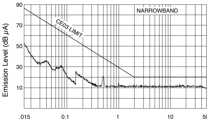
Frequency (MHz), 42 V IN with SFMC28-461 EMI Filter SMHF4207D MIL-STD-461C, CE03
