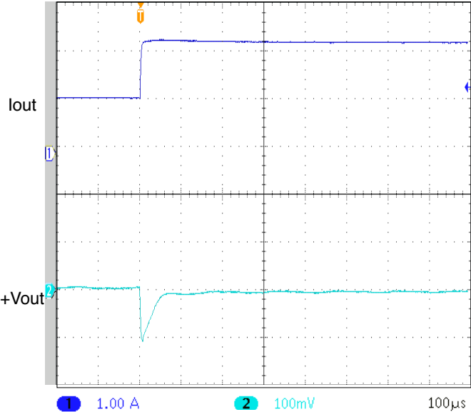
UNITS ARE PER DIVISION SMHF4205S STEP LOAD 50% - 100% FIGURE 23
