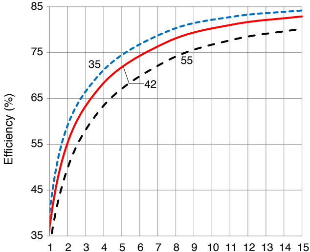
Output Power (Watts) SMHF4215S EFFICIENCY FIGURE 29
