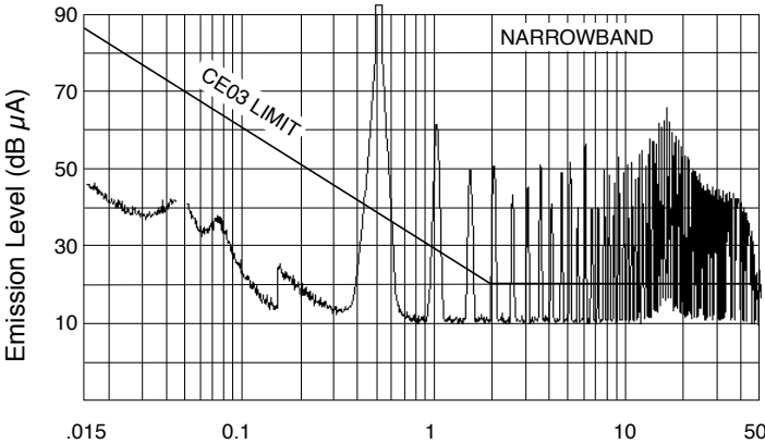
Frequency (MHz), 42 V IN Unfiltered SMHF4215D MIL-STD-461C, CE03 FIGURE 69
