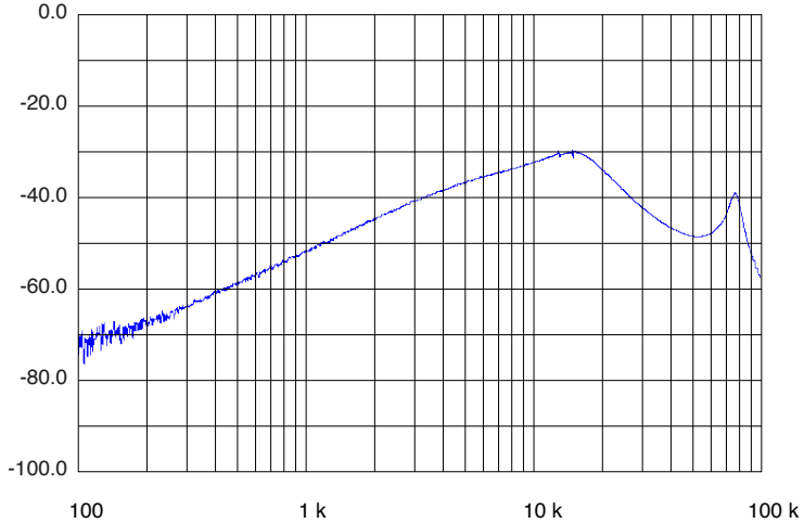
Frequency (Hz), 42 V IN SMHF4207D AUDIO REJECTION
