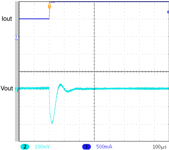
UNITS ARE PER DIVISION SMHF4215S STEP LOAD 50% - 100% FIGURE 35
