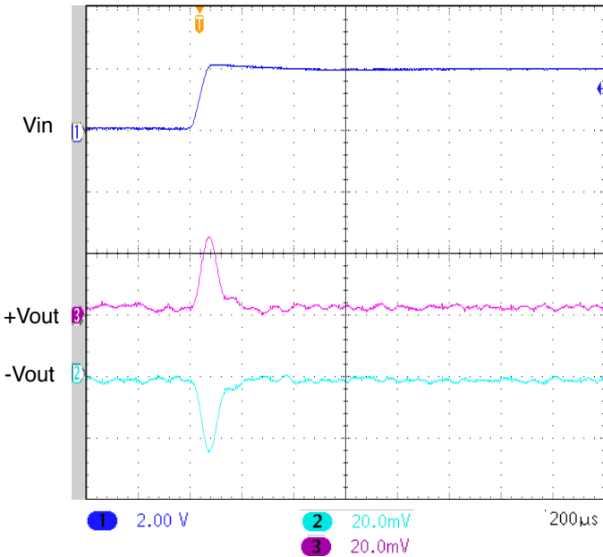
UNITS ARE PER DIVISION SMHF4207D STEP LINE 41 - 43 VOLTS IN FIGURE 62
