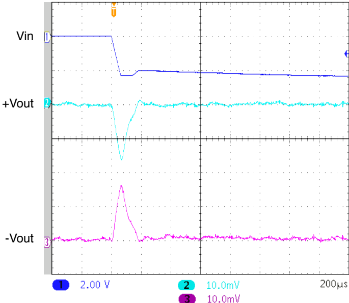
UNITS ARE PER DIVISION SMHF4205D STEP LINE 43 - 41 VOLTS IN FIGURE 50
