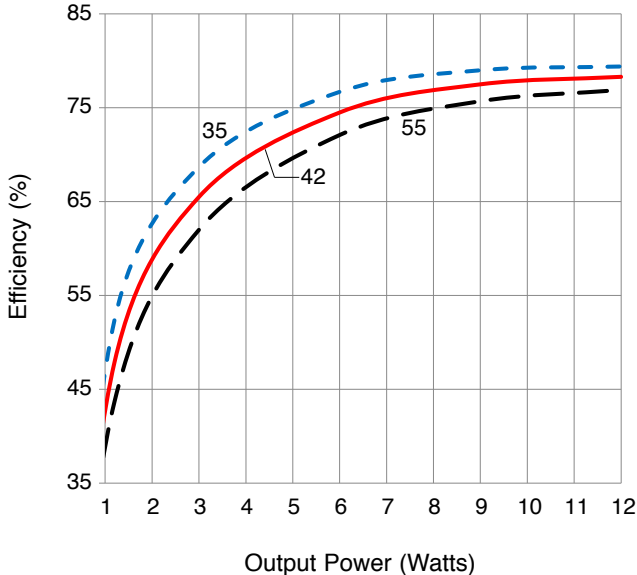
Output Power (Watts) SMHF4205S EFFICIENCY FIGURE 17
