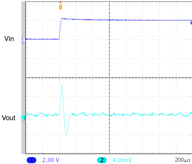
UNITS ARE PER DIVISION SMHF423R3S STEP LINE 41 - 43 VOLTS IN FIGURE 13
