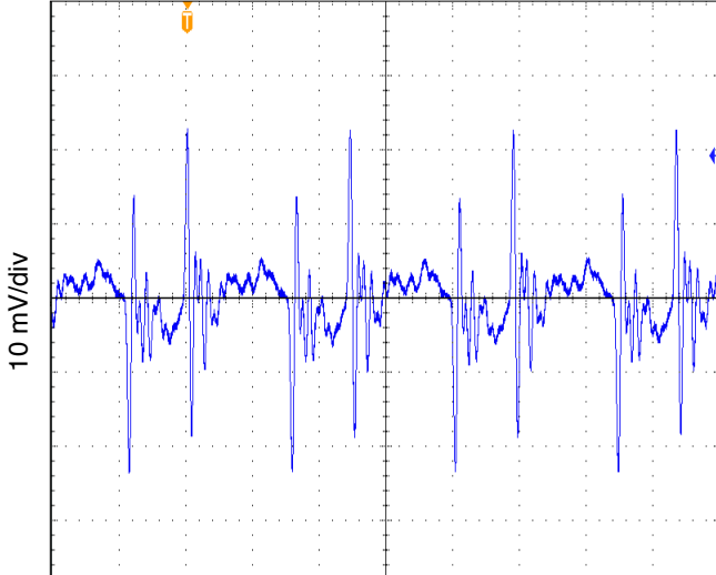
800 nanoseconds/div SMHF4215S OUTPUT RIPPLE 10 MHZ FIGURE 34
