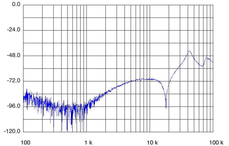
Frequency (Hz), 42 V IN SMHF4205D AUDIO REJECTION FIGURE 42
