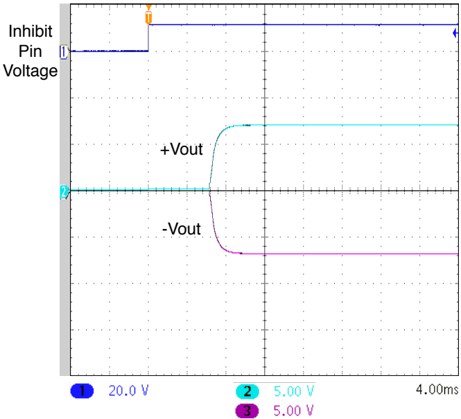
UNITS ARE PER DIVISION SMHF4207D START-UP DELAY NO CAP FIGURE 64
