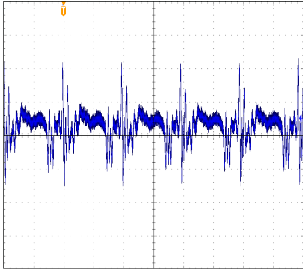
1 \mu s/div SMHF423R3S OUTPUT RIPPLE 10 MHz FIGURE 10
