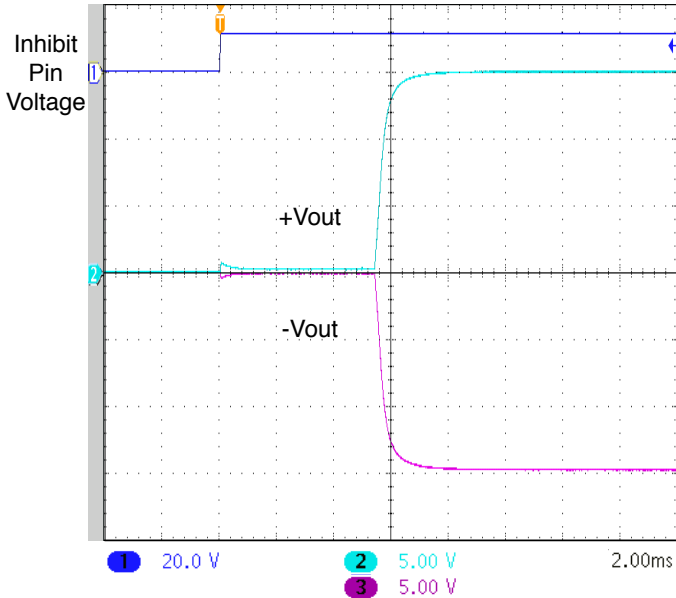
UNITS ARE PER DIVISION SMHF4215D START-UP DELAY NO CAP FIGURE 77
