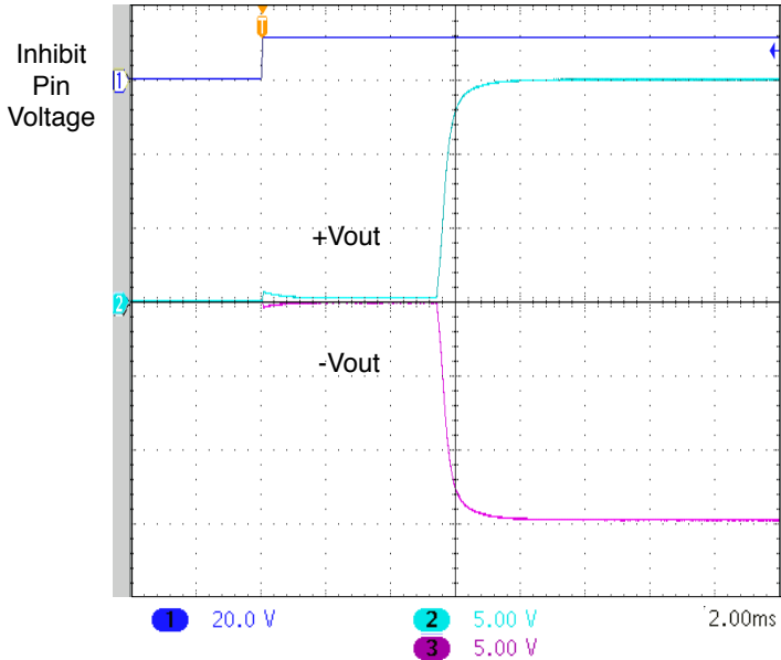
UNITS ARE PER DIVISION SMHF4215D START-UP DELAY WITH 100 µF CAP FIGURE 78
