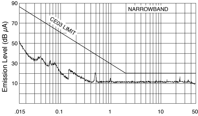
Frequency (MHz), 42 V IN with SFMC28-461 EMI Filter SMHF423R3S MIL-STD-461C, CE03
