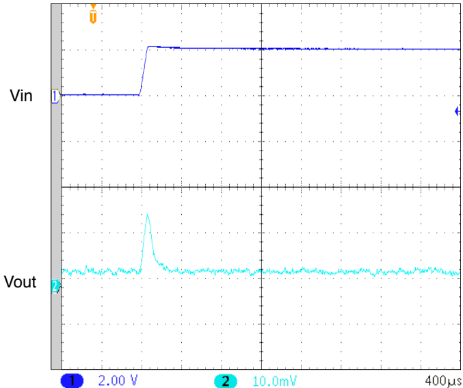
UNITS ARE PER DIVISION SMHF4205S STEP LINE 41 - 43 VOLTS IN FIGURE 25
