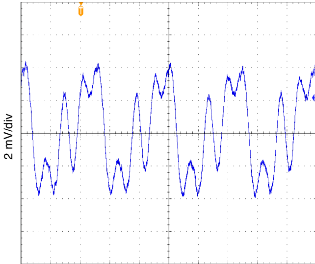
800 nanoseconds/div SMHF4215S OUTPUT RIPPLE 2 MHZ FIGURE 33
