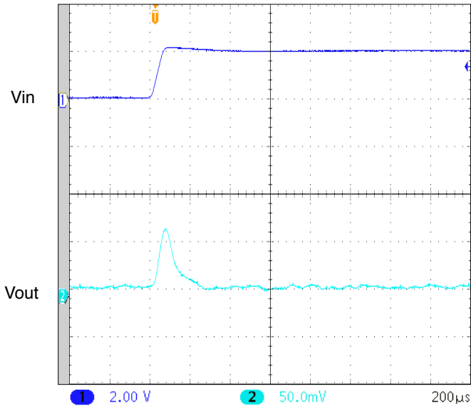
UNITS ARE PER DIVISION SMHF4215S STEP LINE 41 - 43 VOLTS IN FIGURE 37
