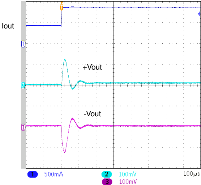
UNITS ARE PER DIVISION SMHF4207D STEP LOAD 50% - 100% FIGURE 60
