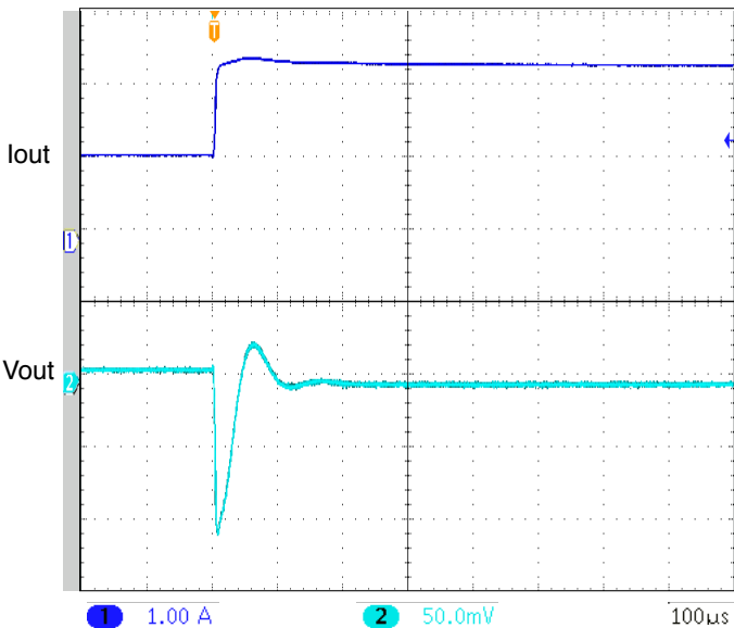
UNITS ARE PER DIVISION SMHF423R3S STEP LOAD 50% - 100% FIGURE 11
