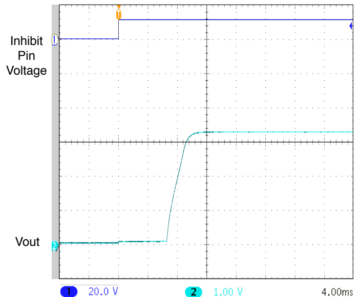
UNITS ARE PER DIVISION SMHF423R3S START-UP DELAY WITH 300 µF CAP FIGURE 16
