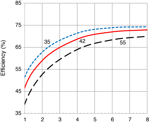
Output Power (Watts) SMHF423R3S EFFICIENCY
