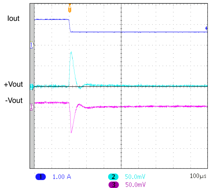
UNITS ARE PER DIVISION SMHF4205D STEP LOAD 100% - 50% FIGURE 48
