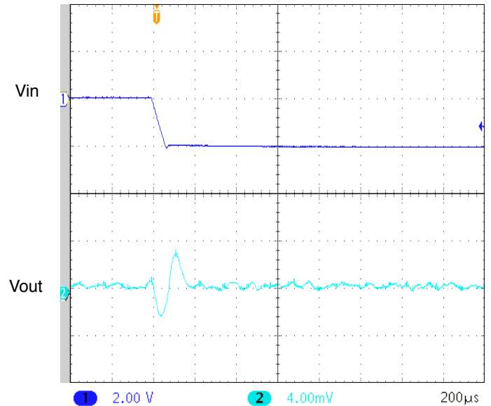
UNITS ARE PER DIVISION SMHF423R3S STEP LINE 43 - 41 VOLTS IN FIGURE 14
