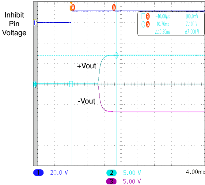
UNITS ARE PER DIVISION SMHF4207D START-UP DELAY WITH 100 µF CAP FIGURE 65
