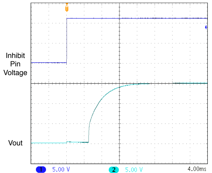
UNITS ARE PER DIVISION SMHF4215S START-UP DELAY WITH 100 µF CAP FIGURE 40
