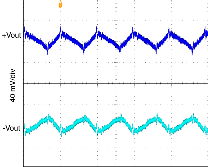
1 microsecond/div SMHF4215D OUTPUT RIPPLE 10 MHZ FIGURE 72
