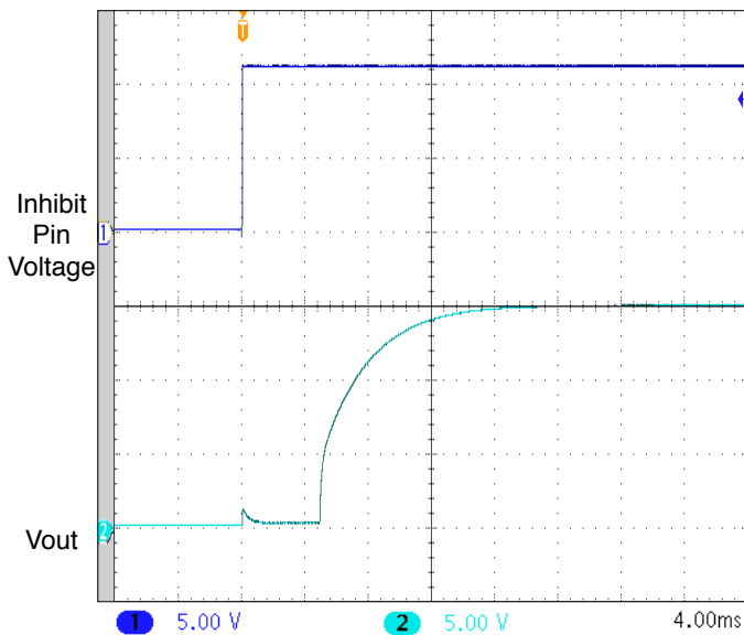
UNITS ARE PER DIVISION SMHF4215S START-UP DELAY NO CAP FIGURE 39
