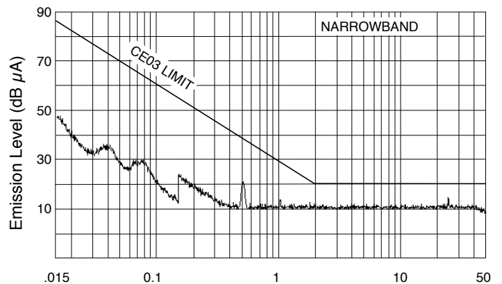
Frequency (MHz), 42 V IN with SFMC28-461 EMI Filter SMHF4205D MIL-STD-461C, CE03 FIGURE 44
