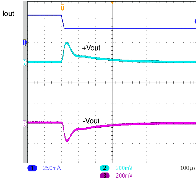
UNITS ARE PER DIVISION SMHF4207D STEP LOAD 100% - 50% FIGURE 74
