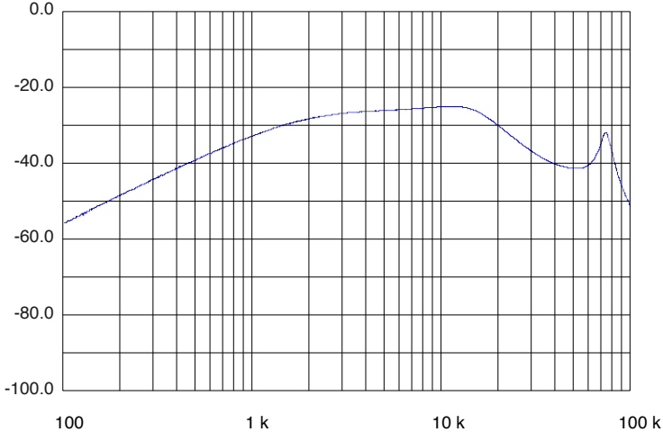
Frequency (Hz), 42 V IN SMHF4215D AUDIO REJECTION FIGURE 68
