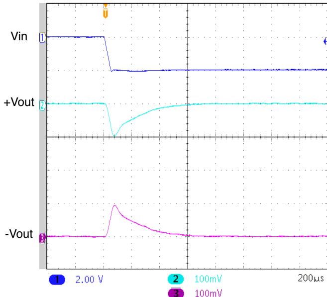
UNITS ARE PER DIVISION SMHF4215D STEP LINE 43 - 41 VOLTS IN FIGURE 76
