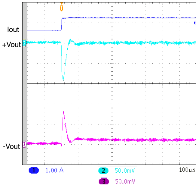
UNITS ARE PER DIVISION SMHF4205D STEP LOAD 50% - 100% FIGURE 47
