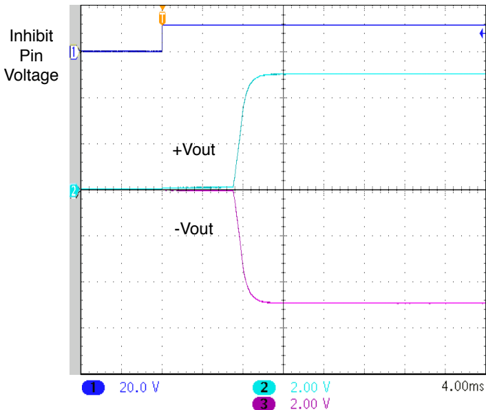
UNITS ARE PER DIVISION SMHF4205D START-UP DELAY WITH 100 µF CAP FIGURE 52
