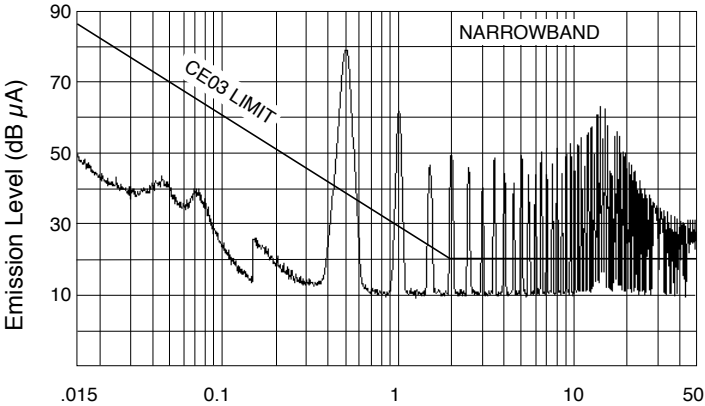
Frequency (MHz), 42 V IN Unfiltered SMHF4207D MIL-STD-461C, CE03
