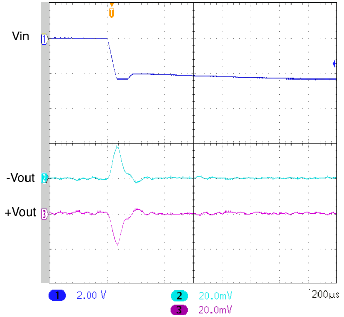
UNITS ARE PER DIVISION SMHF4207D STEP LINE 43 - 41 VOLTS IN FIGURE 63
