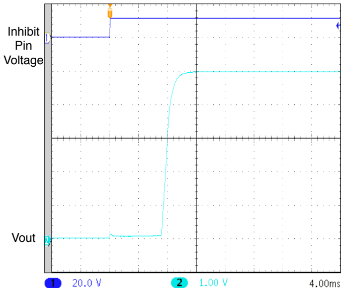
UNITS ARE PER DIVISION SMHF4205S START-UP DELAY NO CAP FIGURE 27
