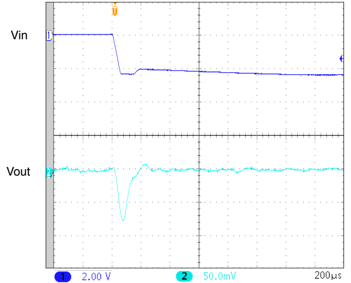
UNITS ARE PER DIVISION SMHF4215S STEP LINE 43 - 41 VOLTS IN FIGURE 38
