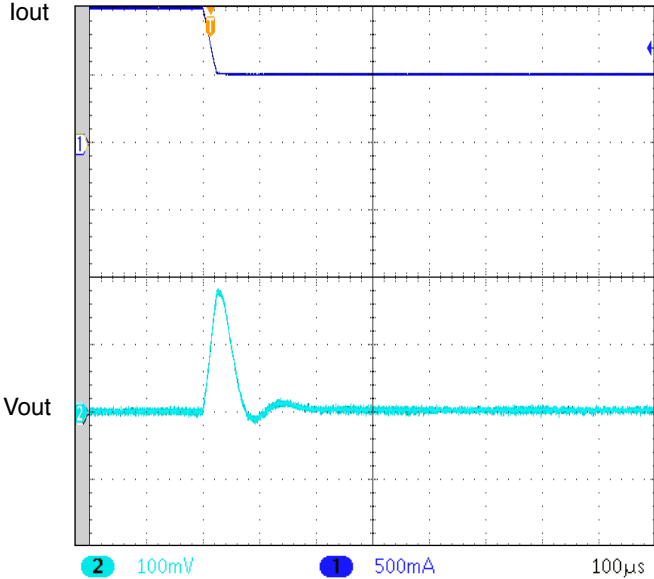
UNITS ARE PER DIVISION SMHF4215S STEP LOAD 100% - 50% FIGURE 36
