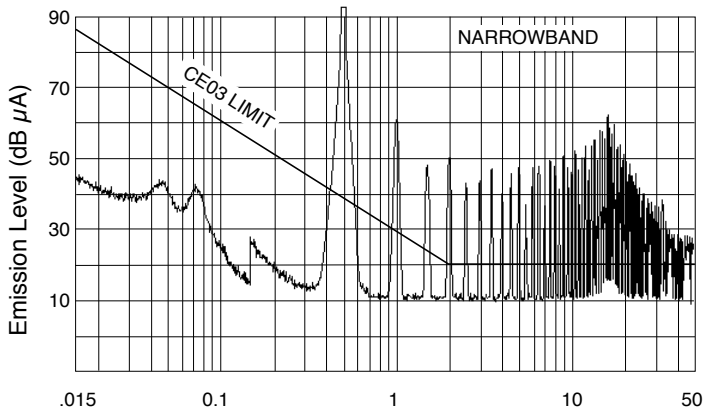
Frequency (MHz), 42 V IN Unfiltered SMHF4205D MIL-STD-461C, CE03 FIGURE 43
