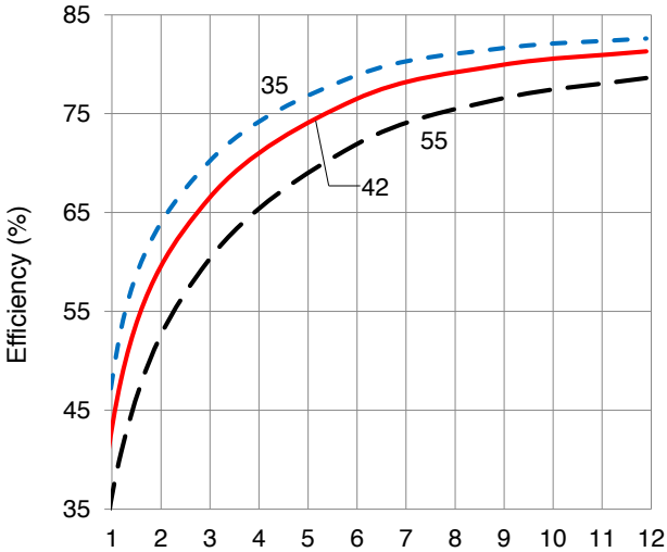
Output Power (Watts) SMHF4207D EFFICIENCY
