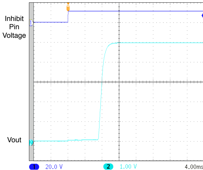
UNITS ARE PER DIVISION SMHF4205S START-UP DELAY WITH 300 μF CAP FIGURE 28
