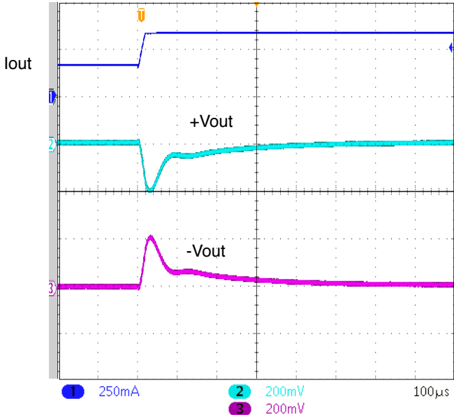
UNITS ARE PER DIVISION SMHF4215D STEP LOAD 50% - 100% FIGURE 73
