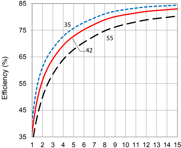
Output Power (Watts) SMHF4215D EFFICIENCY FIGURE 67
