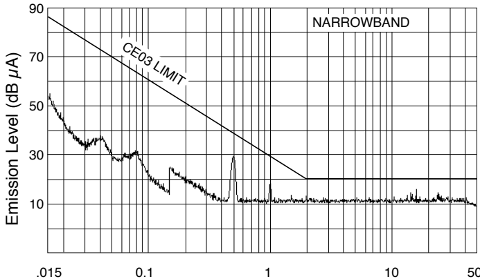
Frequency (MHz), 42 V IN with SFMC28-461 EMI Filter SMHF4215S MIL-STD-461C, CE03 FIGURE 32
