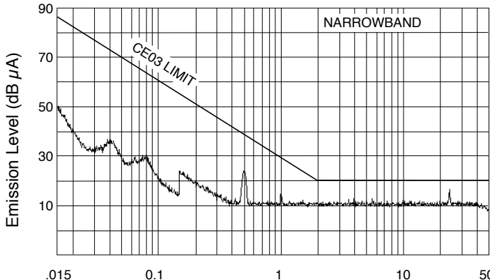
Frequency (MHz), 42 V IN with SFMC28-461 EMI Filter SMHF4215D MIL-STD-461C, CE03 FIGURE 70
