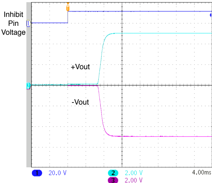
UNITS ARE PER DIVISION SMHF4205D START-UP DELAY NO CAP FIGURE 51
