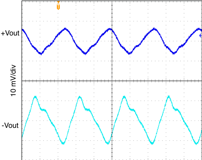
800 nanoseconds/div SMHF4207D OUTPUT RIPPLE 2 MHz FIGURE 58
