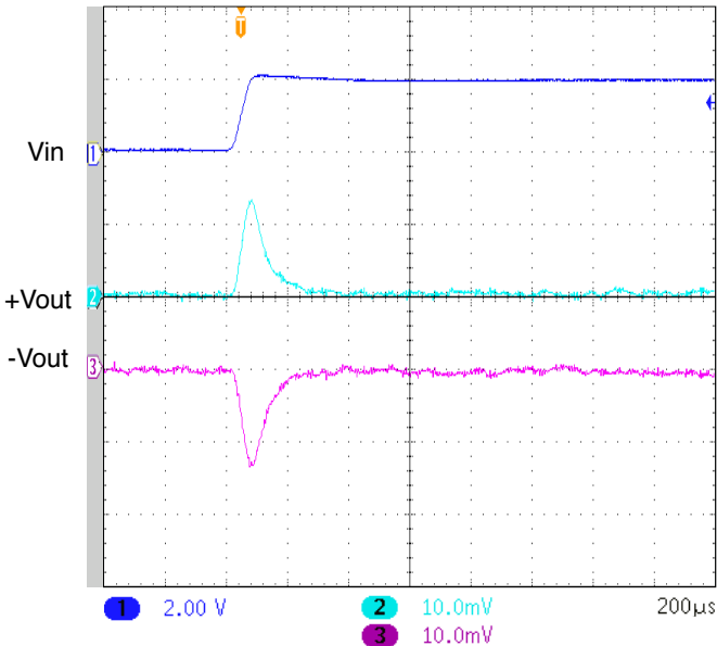
UNITS ARE PER DIVISION SMHF4205D STEP LINE 41 - 43 VOLTS IN FIGURE 49
