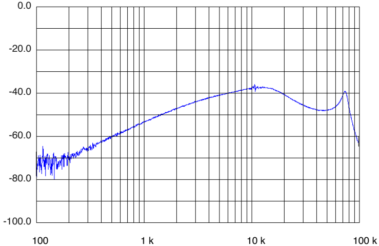
Frequency (Hz), 42 V IN SMHF4205S AUDIO REJECTION FIGURE 18
