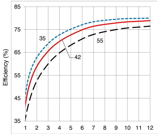
Output Power (Watts) SMHF4205D EFFICIENCY FIGURE 41
