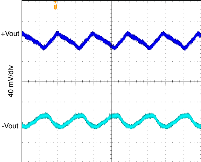
1 microsecond/div SMHF4215D OUTPUT RIPPLE 2 MHZ FIGURE 71
