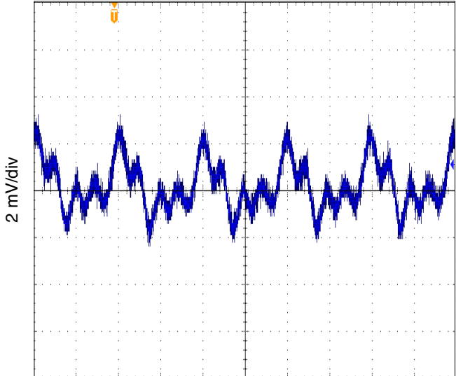
1 μs/div SMHF4205S OUTPUT RIPPLE 2 MHZ FIGURE 21
