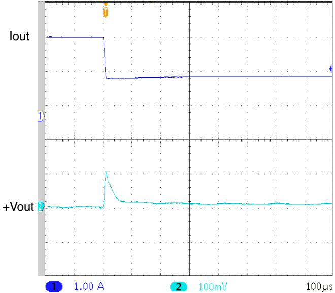
UNITS ARE PER DIVISION SMHF4205S STEP LOAD 100% - 50% FIGURE 24
