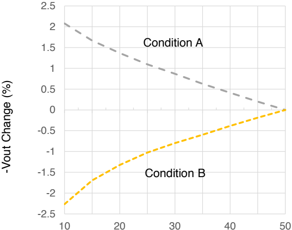
Output Power (%) SMHF4207D EFFICIENCY FIGURE 66
