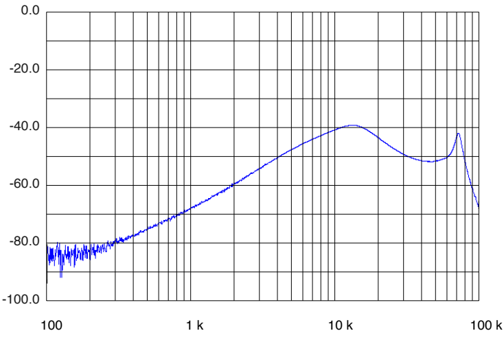
Frequency (Hz), 42 V IN SMHF423R3S AUDIO REJECTION
