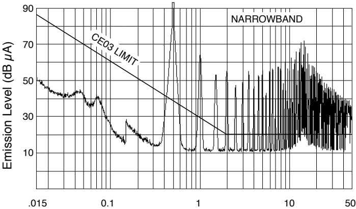
Frequency (MHz), 42 V IN Unfiltered SMHF4215S MIL-STD-461C, CE03 FIGURE 31
