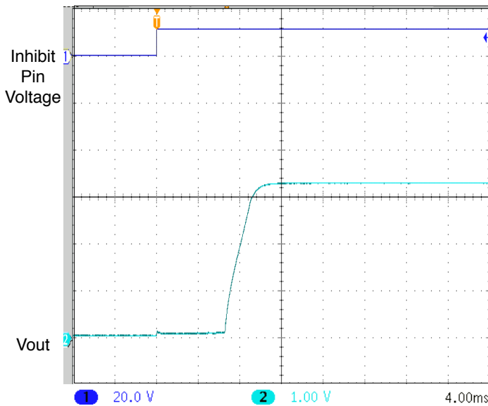
UNITS ARE PER DIVISION SMHF423R3S START-UP DELAY NO CAP FIGURE 15
