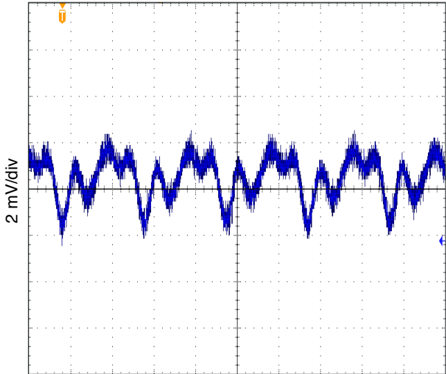
1 \mu s/div SMHF423R3S OUTPUT RIPPLE 2 MHz FIGURE 9
