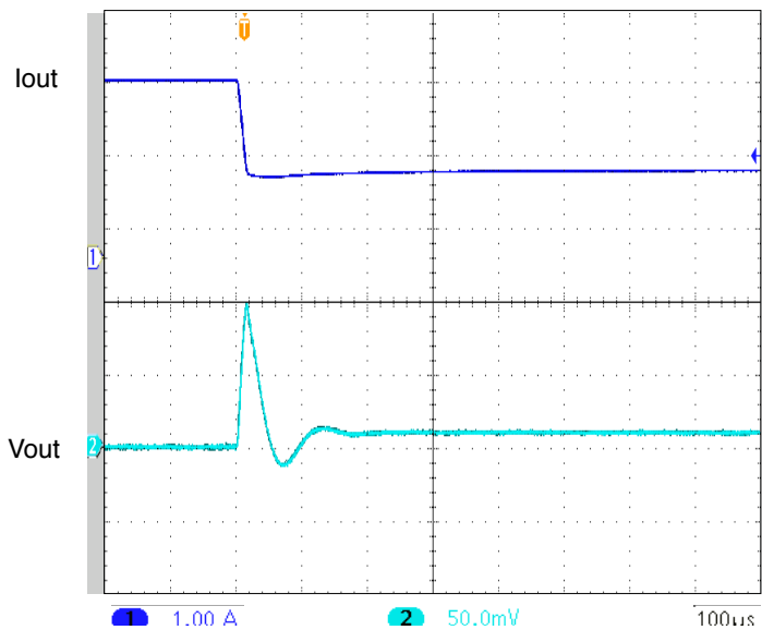
UNITS ARE PER DIVISION SMHF423R3S STEP LOAD 100% - 50% FIGURE 12
