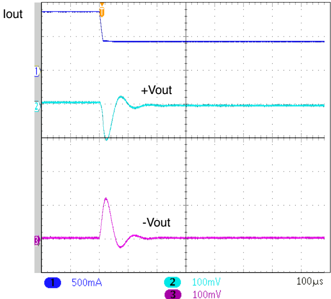
UNITS ARE PER DIVISION SMHF4207D STEP LOAD 100% - 50% FIGURE 61
