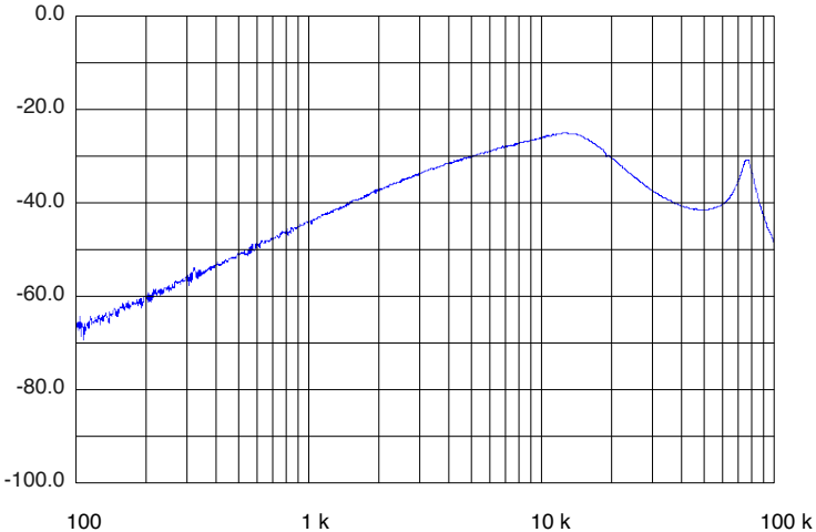
Frequency (Hz), 42 V IN SMHF4215S AUDIO REJECTION FIGURE 30
