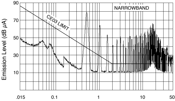
Frequency (MHz), 42 V IN Unfiltered SMHF423R3S MIL-STD-461C, CE03
