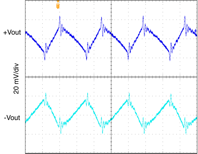
800 nanoseconds/div SMHF4205D OUTPUT RIPPLE 10 MHZ FIGURE 46
