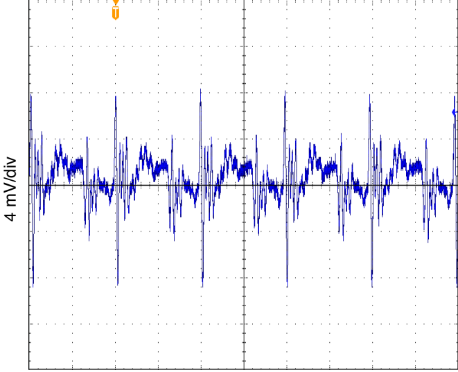
1 μs/div SMHF4205S OUTPUT RIPPLE 10 MHZ FIGURE 22
