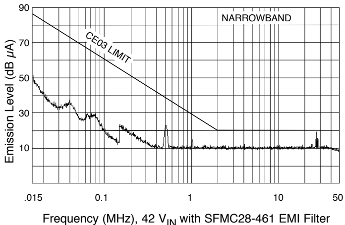
Frequency (MHz), 42 V IN with SFMC28-461 EMI Filter SMHF4205S MIL-STD-461C, CE03
