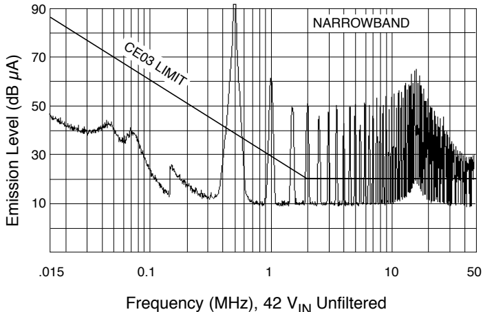
Frequency (MHz), 42 V IN Unfiltered SMHF4205S MIL-STD-461C, CE03
