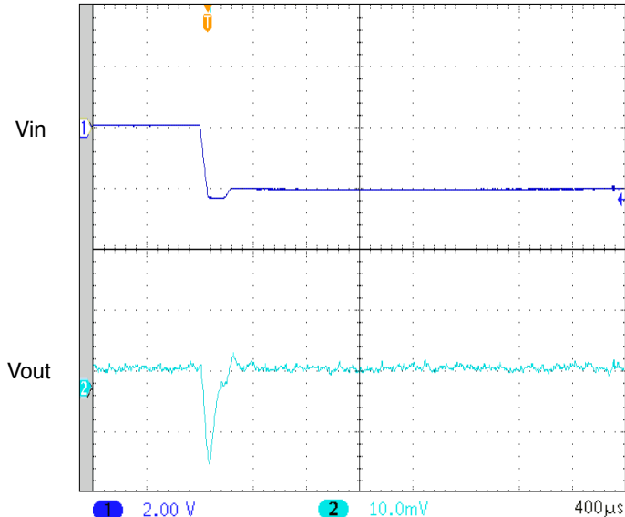
UNITS ARE PER DIVISION SMHF4205S STEP LINE 43 - 41 VOLTS IN FIGURE 26
