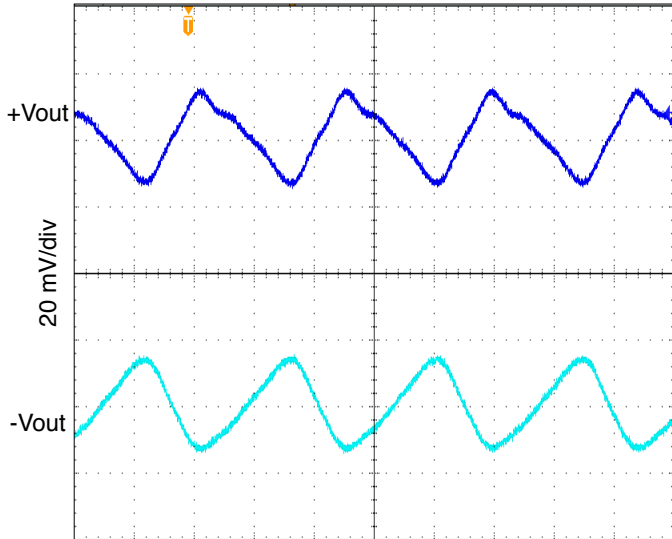
800 nanoseconds/div SMHF4205D OUTPUT RIPPLE 2 MHZ FIGURE 45
