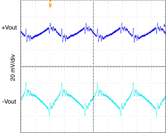
800 nanoseconds/div SMHF4207D OUTPUT RIPPLE 10 MHz FIGURE 59
