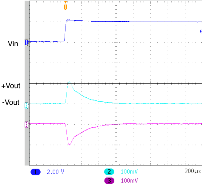
UNITS ARE PER DIVISION SMHF4215D STEP LINE 41 - 43 VOLTS IN FIGURE 75
